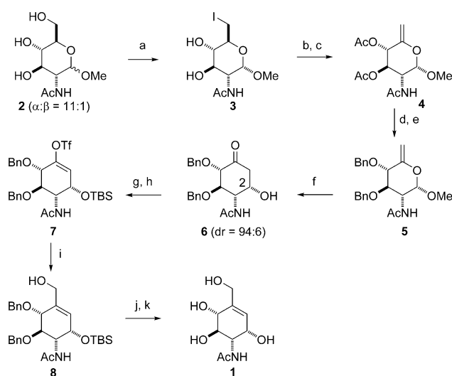
Scheme 1. Synthesis of kirkamide ( 1 ). Reaction conditions: a) Ph 3 P, Imid, I 2 , THF, reflux, 15 min; b) Ac 2 O, pyridine, RT, 24 h; c) AgF, pyridine, RT, 48 h, exclusion of light, 50% over 3 steps; d) NH 3 (gas), MeOH, RT, 3 h; e) NaH, BnBr, DMF, 0°C, 12 h, 36% over 2 steps; f) HgSO 4 dioxane: aq. H 2 SO 4 (5 mM) 2:1, microwave, 60°C, 15 min; g) TBSOTf, 2,6-lutidine, THF, 0°C, 12 h, 63% over 2 steps; h) Comins' reagent, NaHMDS, THF, −78°C, 5 min, 62%; i) Bu 3 SnCH 2 OH, Pd-(PPh 3 ) 4 , LiCl, dioxane, microwave, 105°C, 1 h, 85%; j) TBAF, THF, RT, 3 h, 98%; k) Na/NH 3 (liq), THF, −78°C, 30 min, 59%. Imid: imidazole, THF: tetrahydrofuran, DMF: dimethylformamide, TBS: tert -butyldimethylsilyl, HMDS: hexamethyldisilazane. TBAF: tetra- n -butylammonium fluoride.
